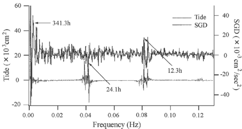
Figure 5: Time series analysis (FFT method) of long-term SGD measurements and tides in Osaka Bay, Japan, from May 29 to August 23, 2001. The main SGD frequencies correspond to semi-diurnal (12.3 h), diurnal (24.1 h), and bi-weekly (341.3 h) lunar cycles (reproduced from Taniguchi, 2002).
