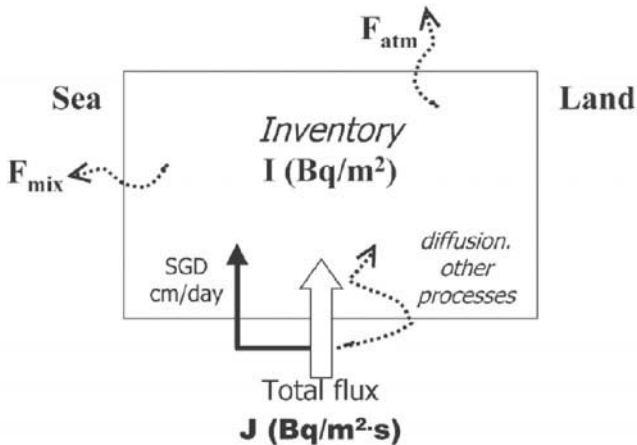
Figure 3: Conceptual model of use of continuous radon measurements for estimating submarine groundwater discharge in a coastal zone. The inventory refers to the total amount of excess ^{222}\text{Rn} per unit area. Decay is not considered because the fluxes are evaluated on a very short (1–2 hours) time scale relative to the half-life of ^{222}\text{Rn} (Reproduced from Burnett and Dulaiova, 2003).
